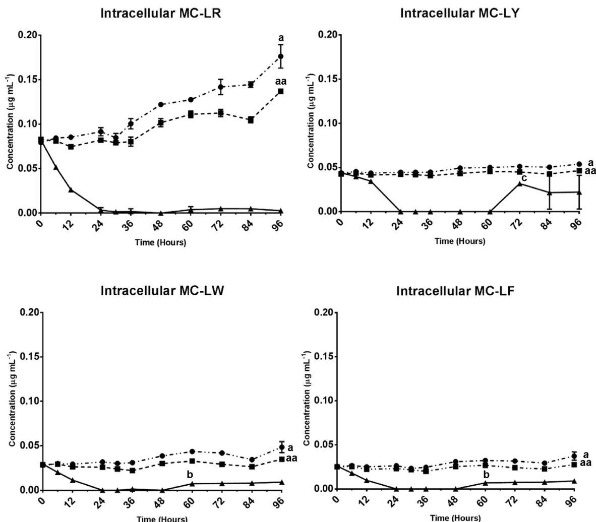
Fig. 7. Removal of intracellular MC-LR, -LY, -LW and -LF after exposure to 0 (●), 5 (■) and 20 (▲) mg L -1 hydrogen peroxide over 96 h under cool white fluorescent lights of 10.5 μmol photons m -2 s -1 . a, aa = significantly different from T 0 ; b = significantly different from 48 h; c = significantly different from 60 h (n = 3, error bars = σ -1 ).
