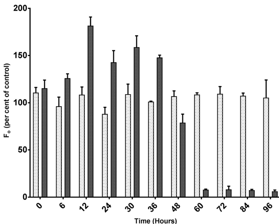
Fig. 6. Microcystis aeruginosa PCC 7813 minimal fluorescence (indicative of chlorophyll \alpha ) results (percentage of the control) after being treated for 96 h with different \text{H}_2\text{O}_2 dosages ( \square ) 5 and ( \blacksquare ) 20 \text{ mg L}^{-1} under cool white fluorescent lights of 10.5 \mu\text{mol photons m}^{-2} \text{ s}^{-1} with different dosages of \text{H}_2\text{O}_2 ( n = 3 , error bars = \sigma_{-1} ).
